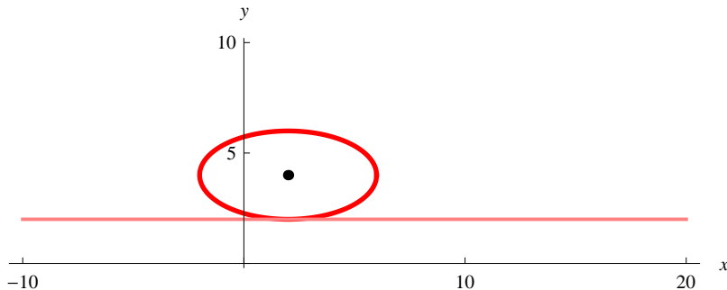
Figure 1.1: The original ellipse and the horizontal line it will roll along.
