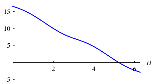
Figure 1.2: Difference of 2 and the arclength of the ellipse.
