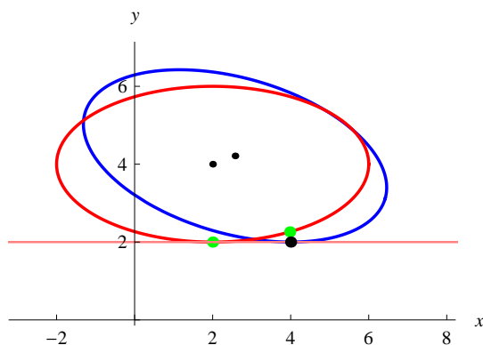
Figure 1.7: Original ellipse and the rotated ellipse, both in the correct positions.
