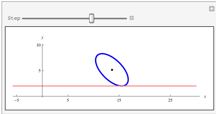
Figure 1.8: The 27th frame in the animation of rolling the ellipse.
