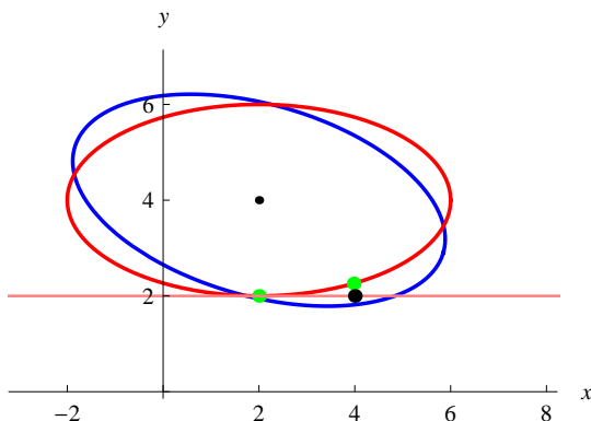
Figure 1.6: Original ellipse and the rotated ellipse, both at center (2, 4).
