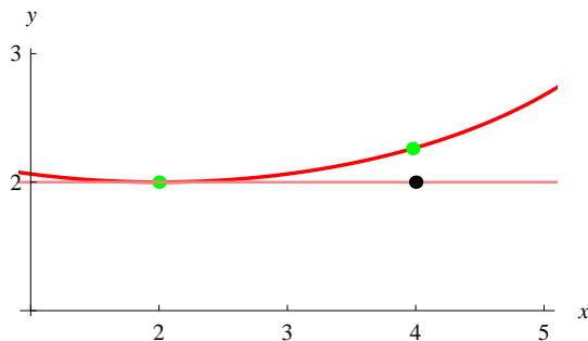
Figure 1.4: Close-up of Figure 1.3 near the desired point of rotation.
