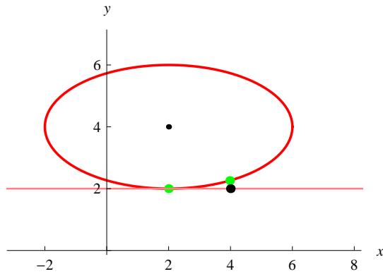
Figure 1.3: Original point on the ellipse which touches the line, and the new point which will touch the line after rolling two units to the right.
