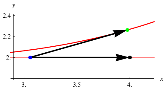
Figure 1.5: The vectors needed to compute the angle of rotation for the first step in the rolling.
